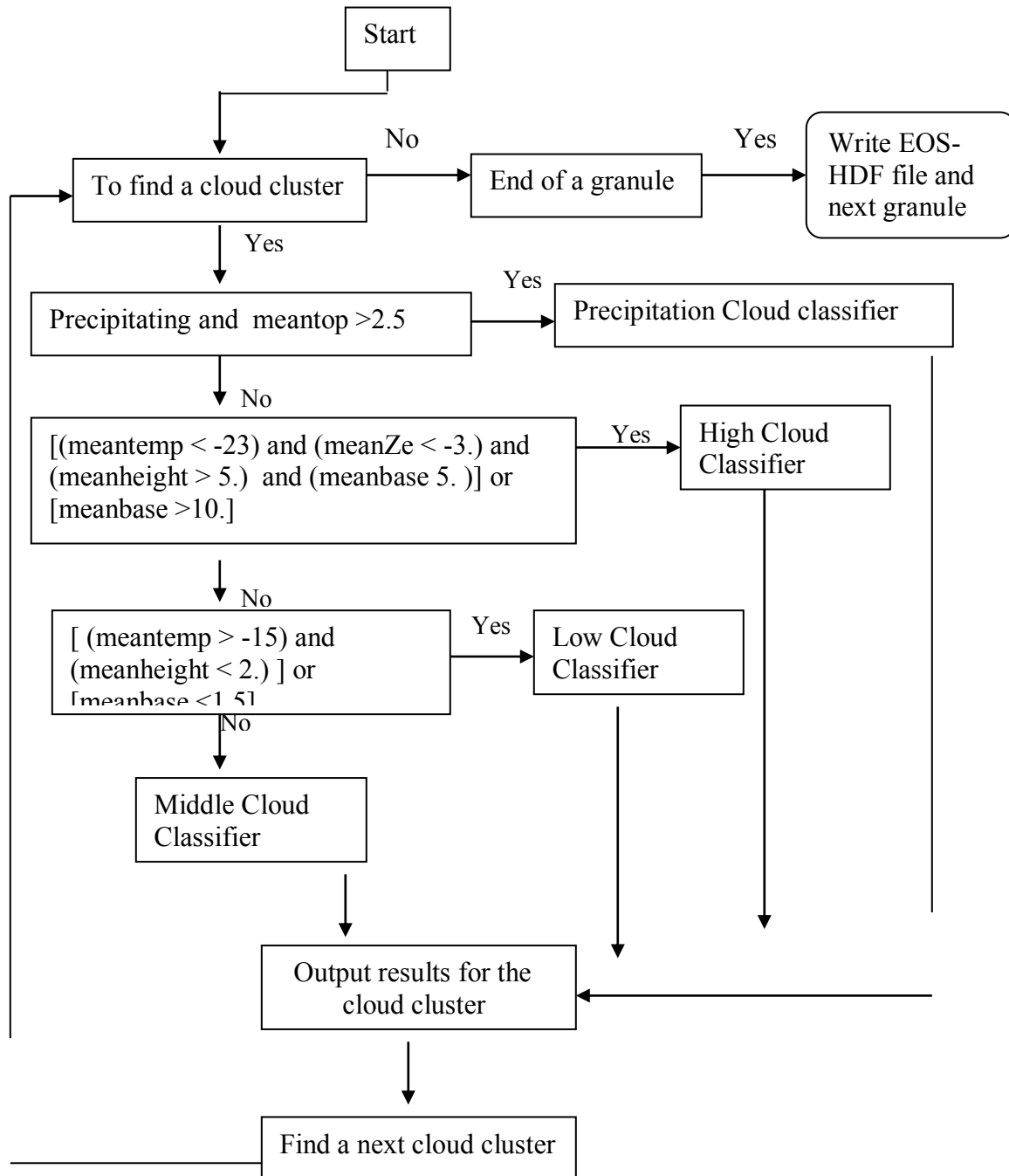
Figure 4: The high level flowchart of cloud scenario classification algorithm
