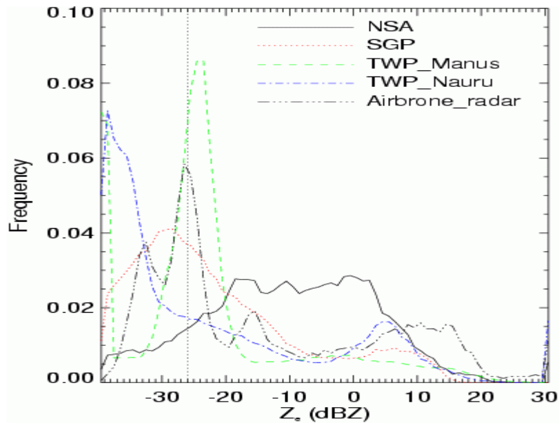
Figure 6: The frequency distribution of the maximum radar reflectivity factor within 2 km above surface from MMCR measurements at SGP, NSA and TWP sites and airborne cloud radar measurements. The vertical dashed line indicates the -26 dBZ.
