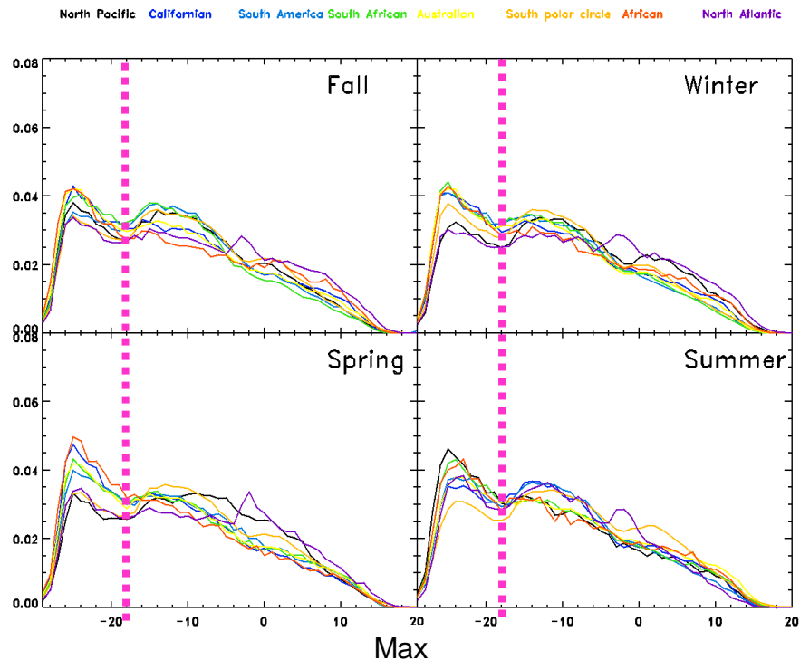
Figure 12. Maximum Z_e distribution for marine clouds with cloud top below 3.5 km over 8 Sc cloud occurrence regions (color coded). The Z_e values presented here are non-attenuation corrected CloudSat measurements from June 2006 to April 2007.
