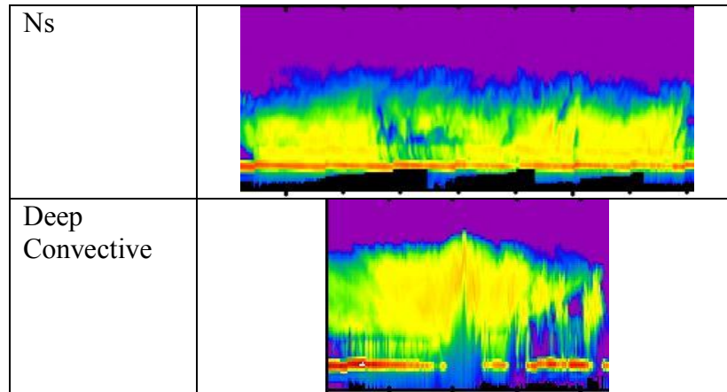
Figure 13. Typical examples of different cloud types observed by CloudSat. Horizontal axis represents distance along CloudSat track, and vertical axis represents cloud altitude. Surface height is indicated by strong signals (red or white colors) except regions strongly attenuated by precipitation.
