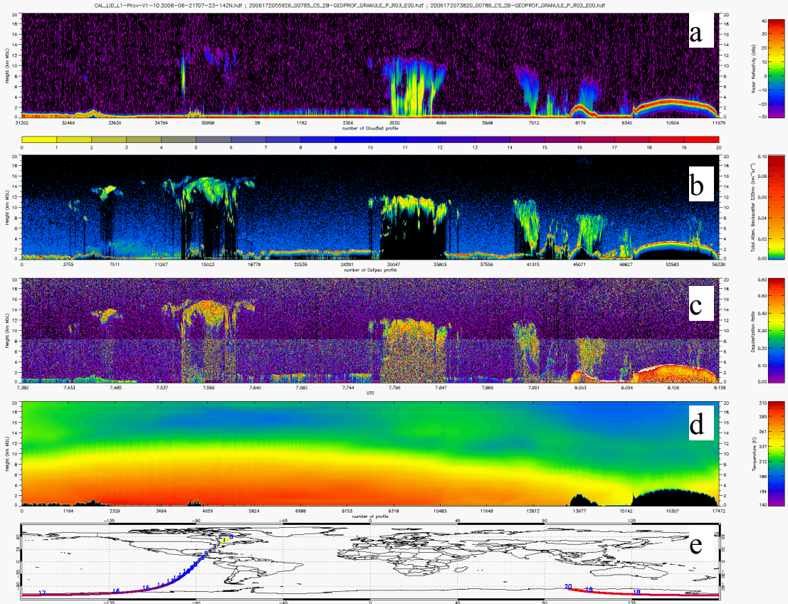
Figure 2: Colocated CloudSat radar (a), CALIPSO attenuated backscattering coefficient (b) and depolarization ratio (c), ECMWF temperature profile (d), and CloudSat track (e).
