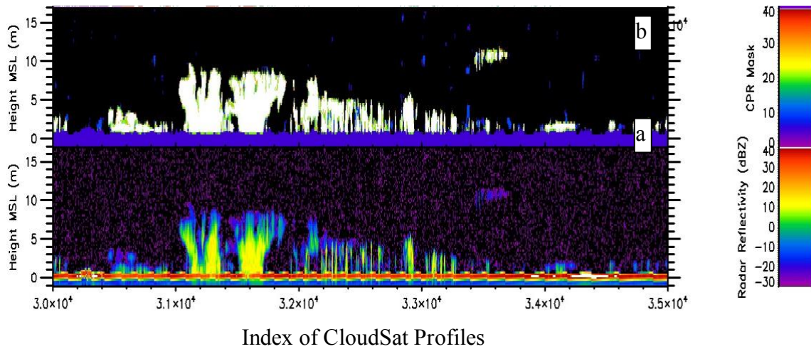
Figure 1: An example of CloudSat measured radar reflectivity factor (a) and cloud mask results (b) from 2B-GEOPROF product.
