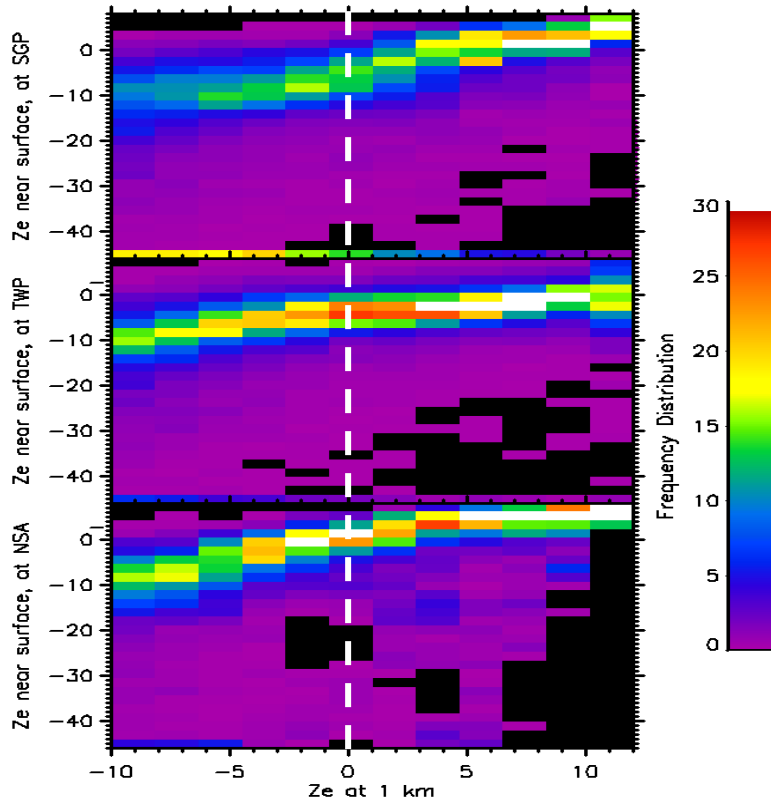
Figure 8. The correlation of near surface radar signals with signals at 1 km based on ARM surface observations at three different climate regions
