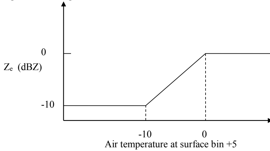
Figure 9, Z_e threshold for precipitation detection based on near surface CloudSat signal intensity and air temperature.
